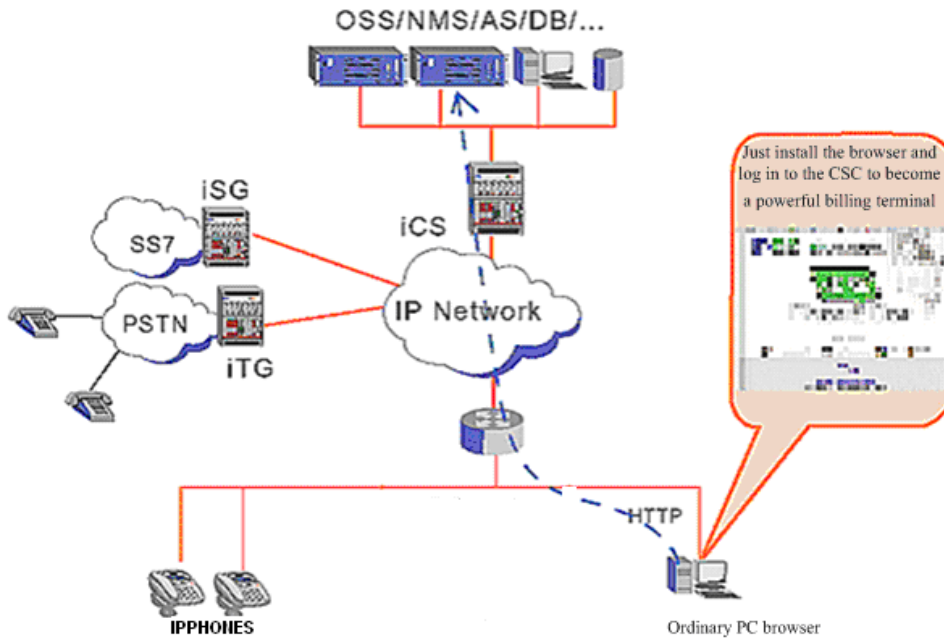
Operator IP Telephone Bar System Architecture (Catogory-5 Cable)
